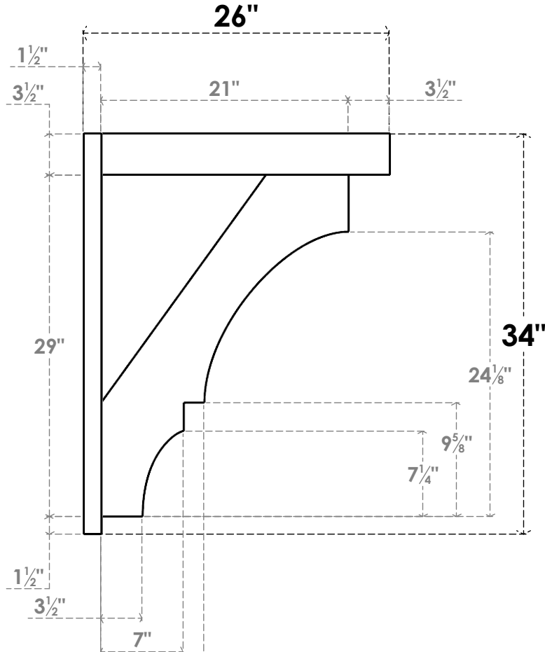
SIDE PROFILE
